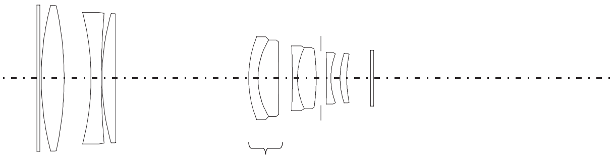
Internal focussing
